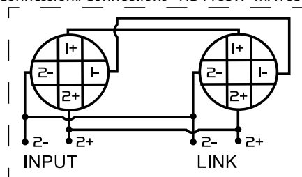
Connessioni/Connections - HD118SW- MA18SP
