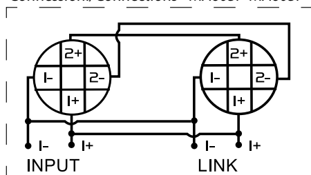
Connessioni/Connections - MA605P-MA605P
