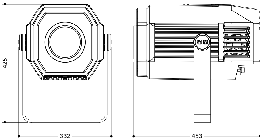
Technical drawing
